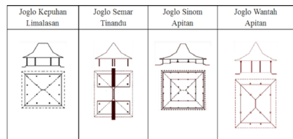
Gambar 8 Macam denah rumah Joglo Sumber: google.com. 2018
