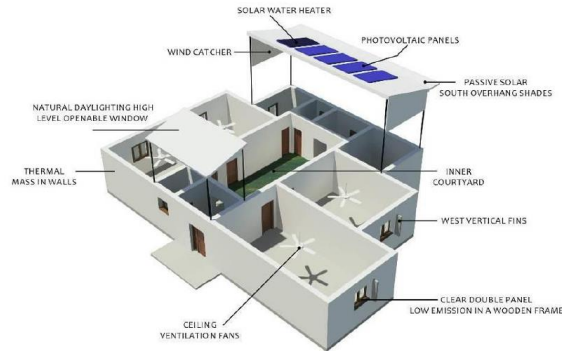
Gambar 5. Desain green building [22]
